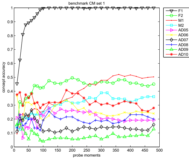
Figure 2: CM, training set F1.
