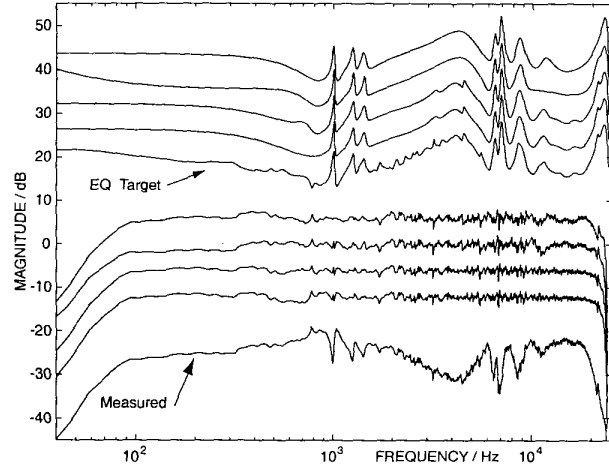
Figure 4: Equalized responses and Kautz equalizers constructed partly or purely from observing original and target responses. The Kautz filter orders are 20, 23, 34 and 32, from top to bottom, in respective block for the equalizers and the simulated equalization.
