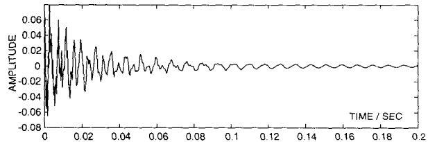
Figure 5: Measured impulse response of an acoustic guitar body.
